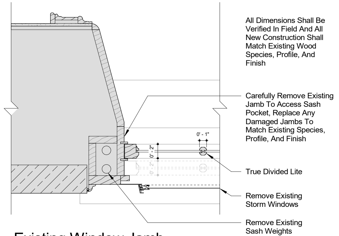
Existing Window Jamb 1 1/2" = 1'-0"
