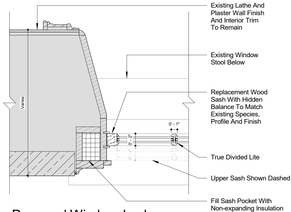
Proposed Window Jamb 1 1/2" = 1'-0"
